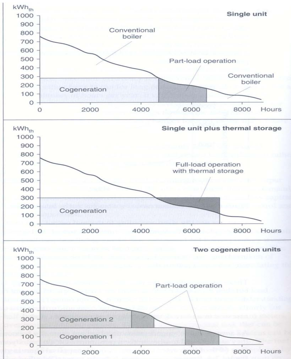
Thermal load duration curve for a hospital: a) for a single 300 \text{kW}_{\text{th}} cogeneration unit; b) for the same unit with thermal storage; c) for two 200 \text{kW}_{\text{th}} cogeneration units.
